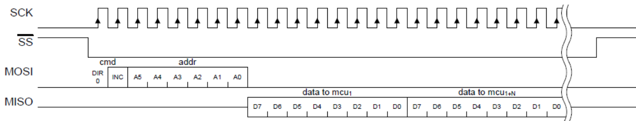
Figure 3 – SPI Incrementing Burst Read Sequence
