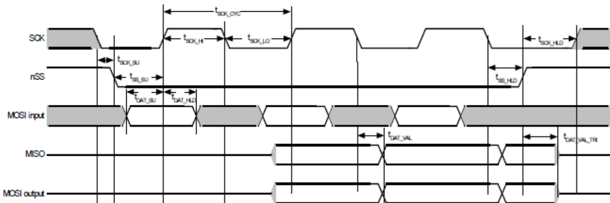
Figure 6 – SPI Timing
