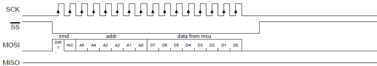
Figure 4 – SPI Single Write Sequence
