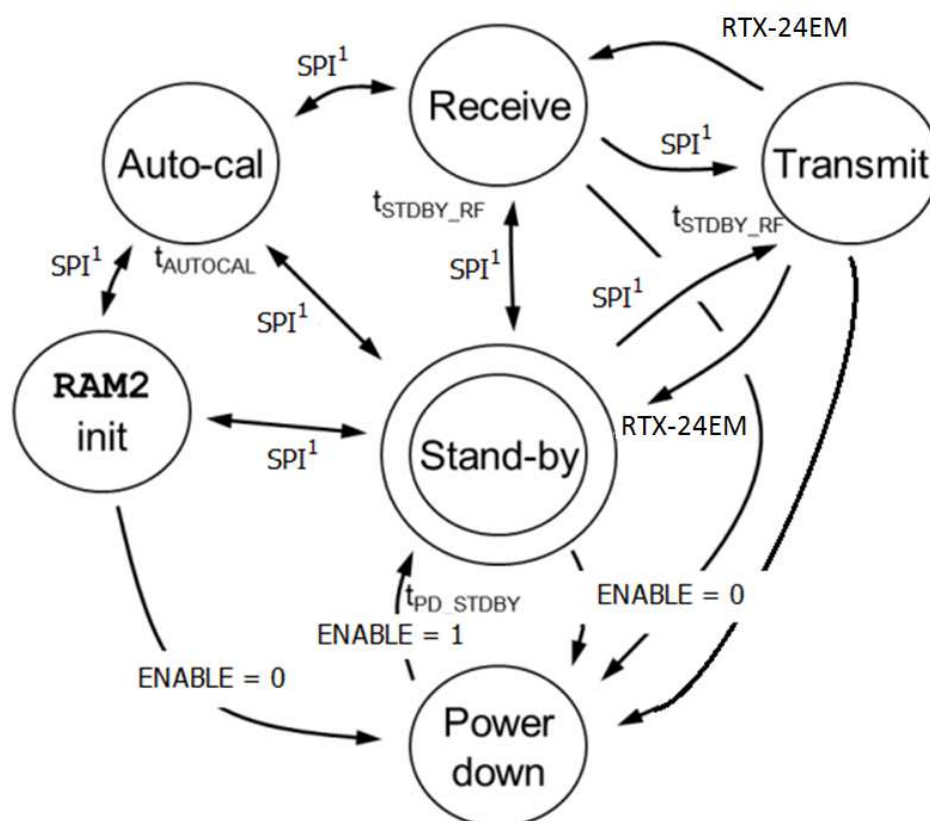
Figure 1: RTX-24EM-HP Functional Overview
