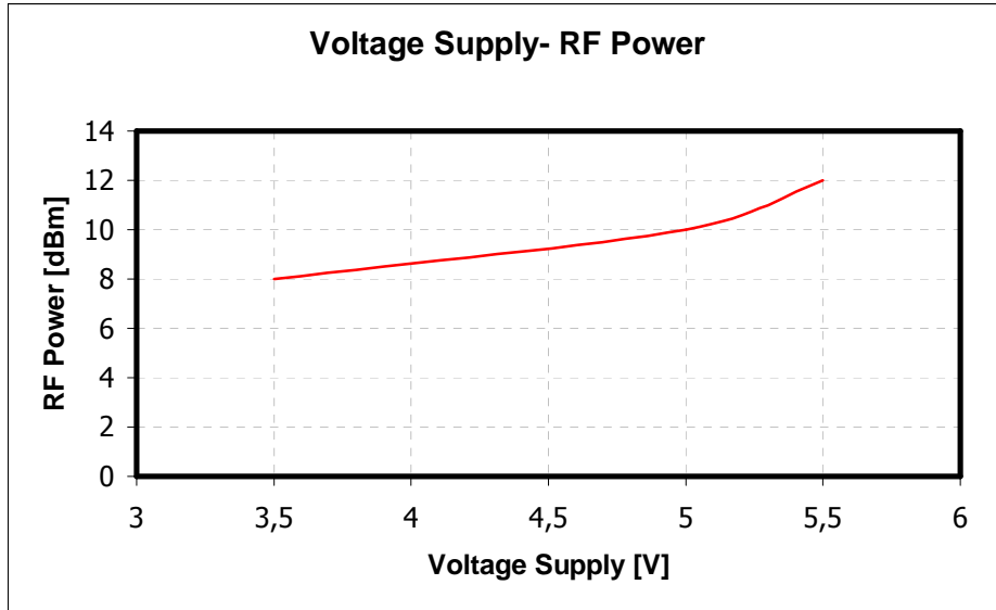
Fig. 3 RF Power Vs Voltage Supply
