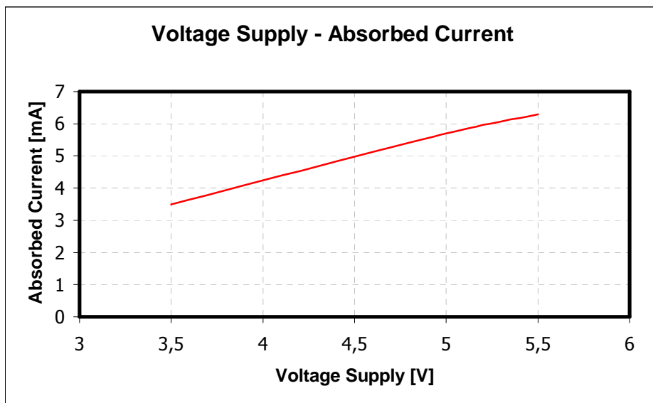
Fig. 4 Absorbed Current Vs Voltage Supply The curve has been obtained by the testing system shown in Fig.1.
