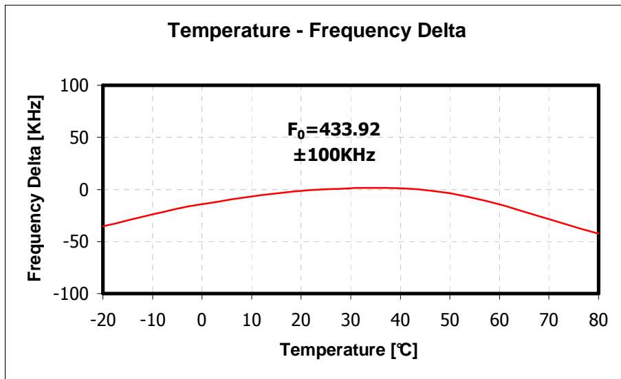
Fig. 7 Frequency Delta Vs Temperature
