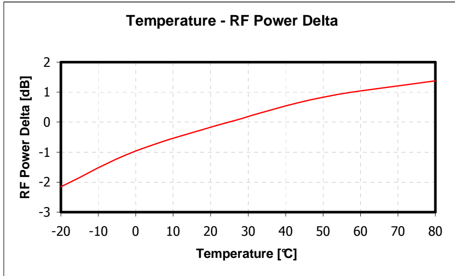
Fig. 5 RF Power Delta Vs Temperature
