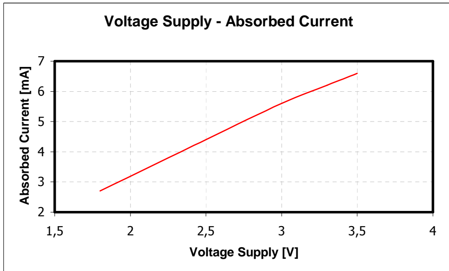
Fig. 4 Absorbed Current Vs Voltage Supply
