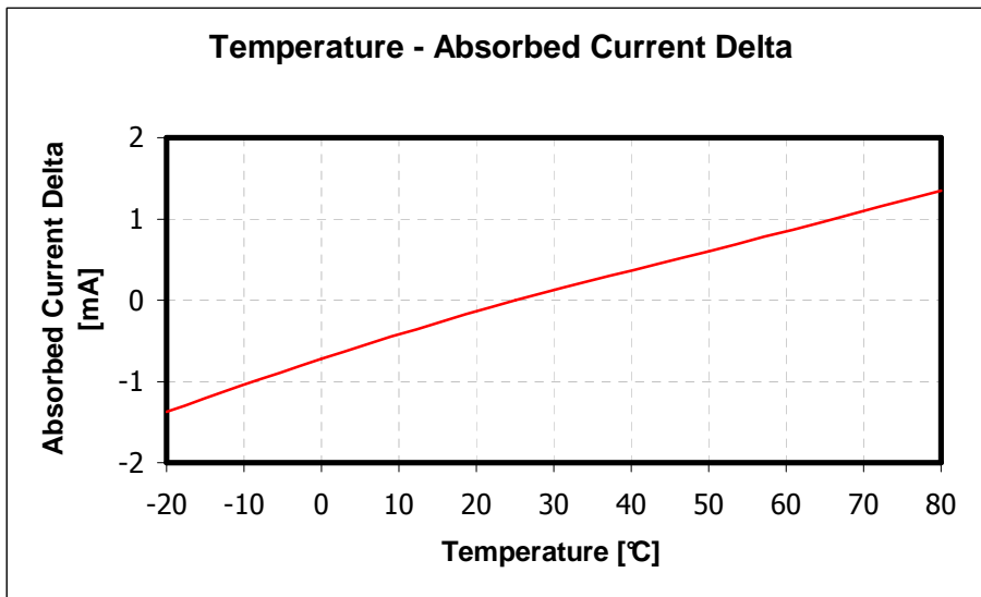
Fig. 6 Absorbed current Delta Vs Temperature
